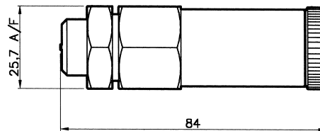
1/8" AL Variante 2C, 3C, 3D, 4D and 4F
